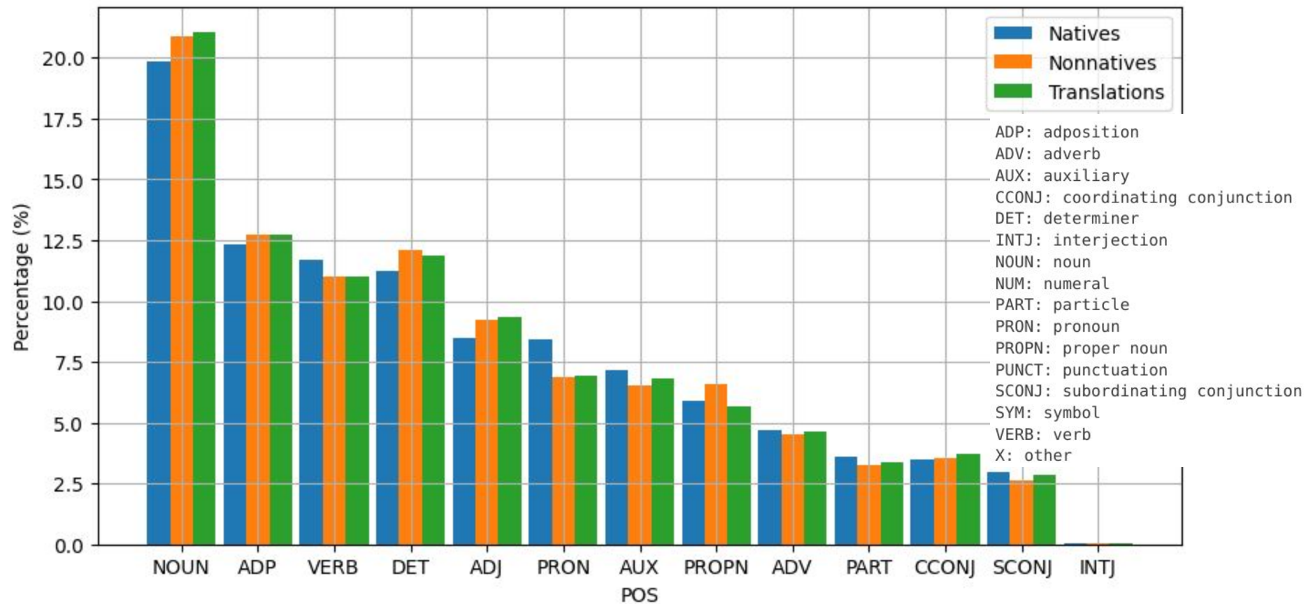
POS distribution
