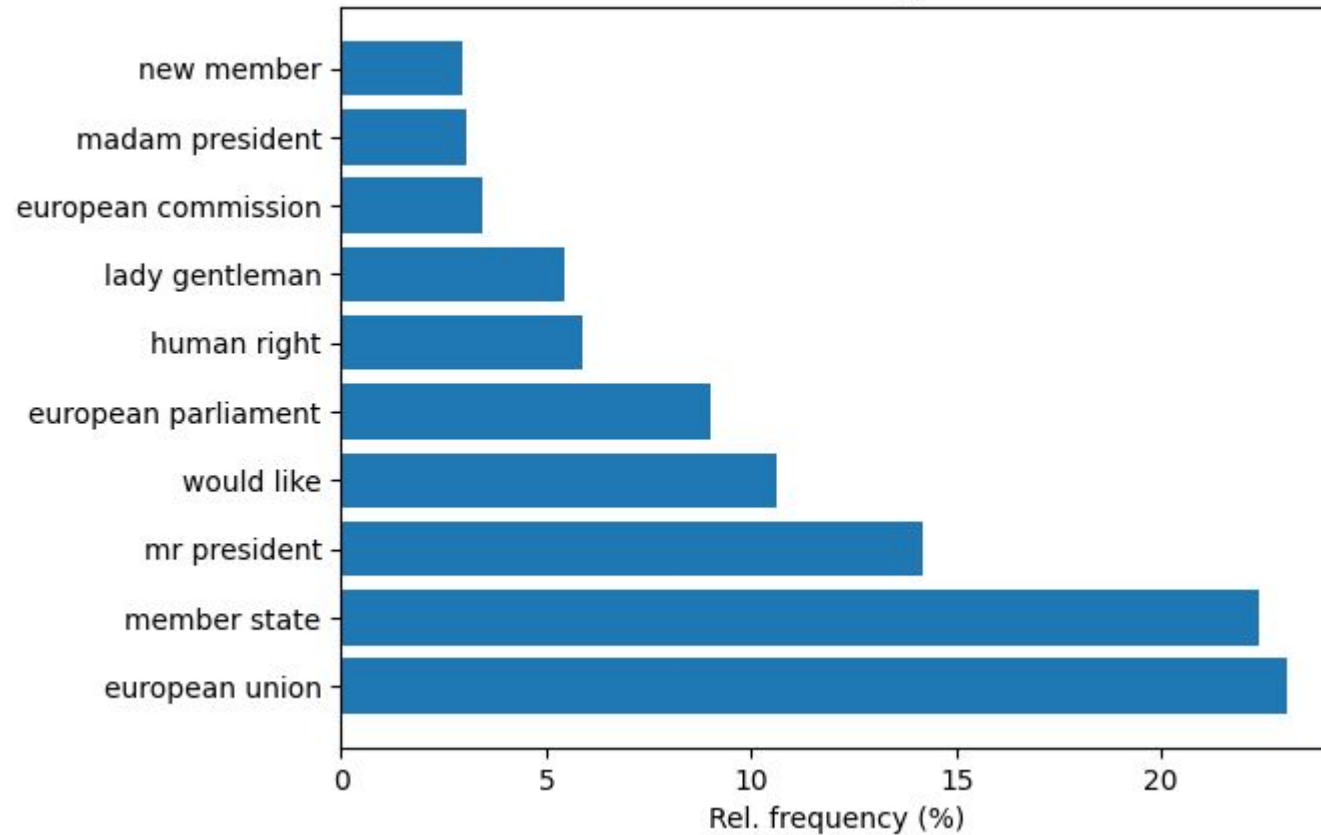
Translations bigrams
